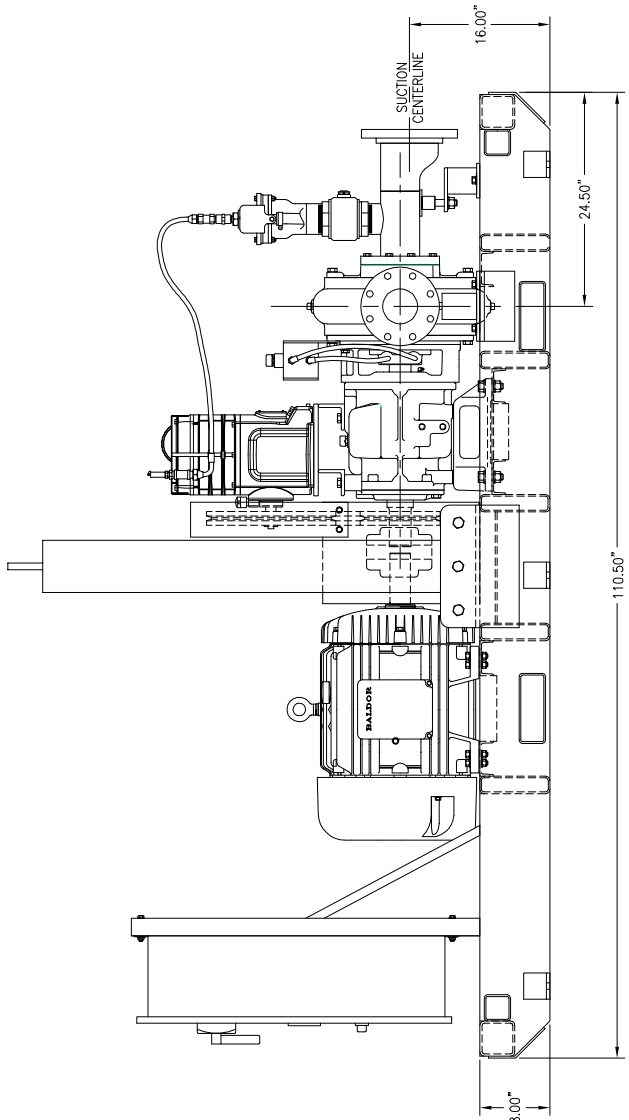
SIDE VIEW
